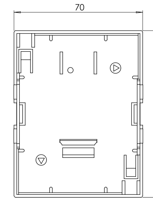
SURFACE-12 (INSIDE)
