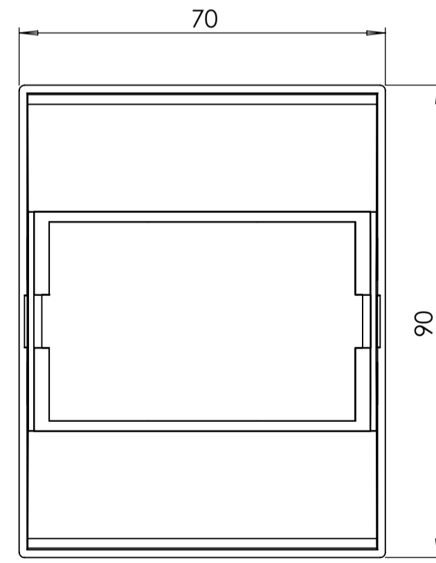
SURFACE-6 (INSIDE)
