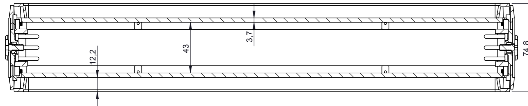
SECTION B-B
