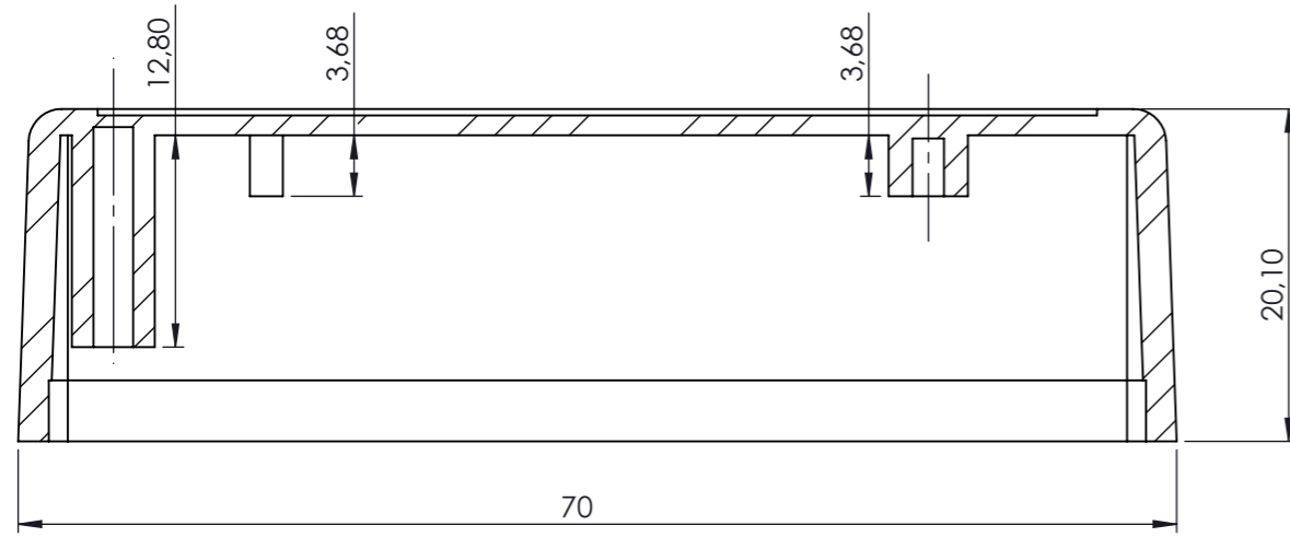
SECTION B-B
